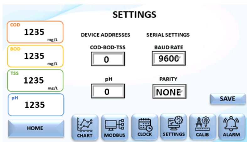
Figure 10 – Settings Screen
