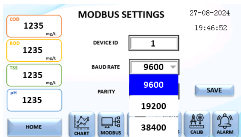
Figure 6 - Modbus Menu
